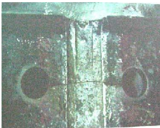
FIG. 52 : 422 - WELDING, THERMIT JOINT HORIZONTAL CRACK
