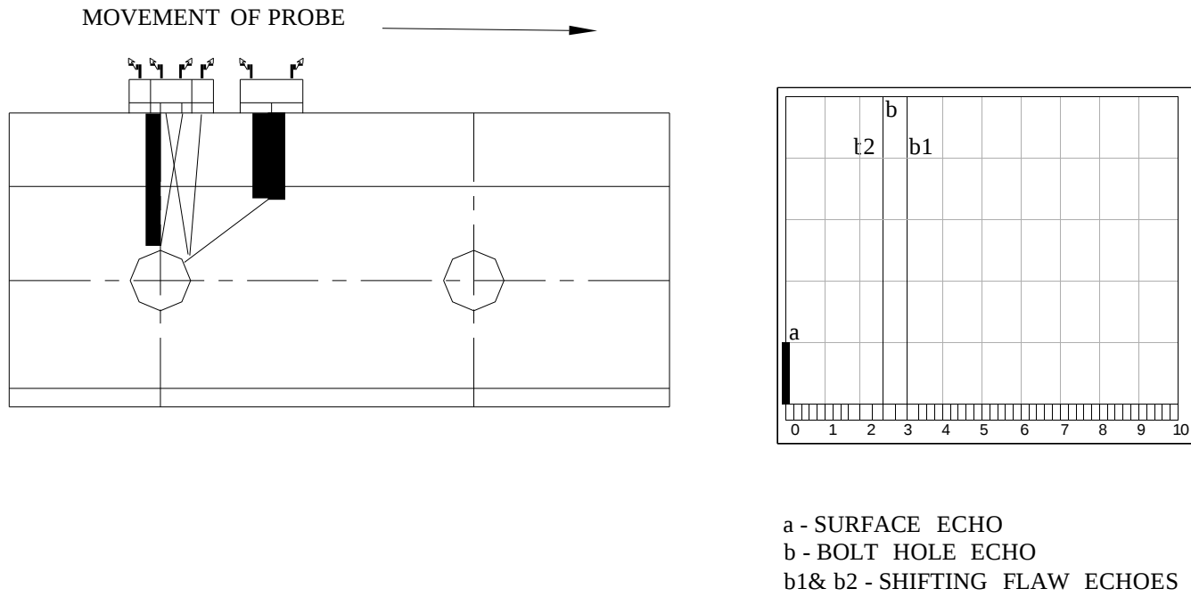
FIG. 16: BOLT HOLE WITH CRACK (TYPE 135,235,0° PROBE)
