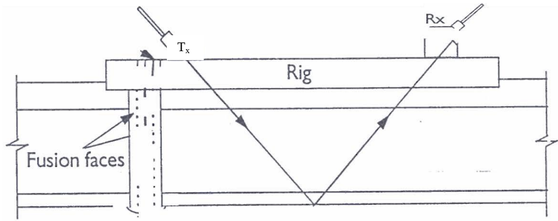
Fig.22(b): Sensitivity setting using 45 0 tandem probe
