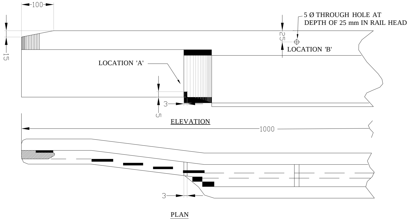
FIG. 26(b) : STANDARD TEST PIECE (SEJ STOCK RAIL)
