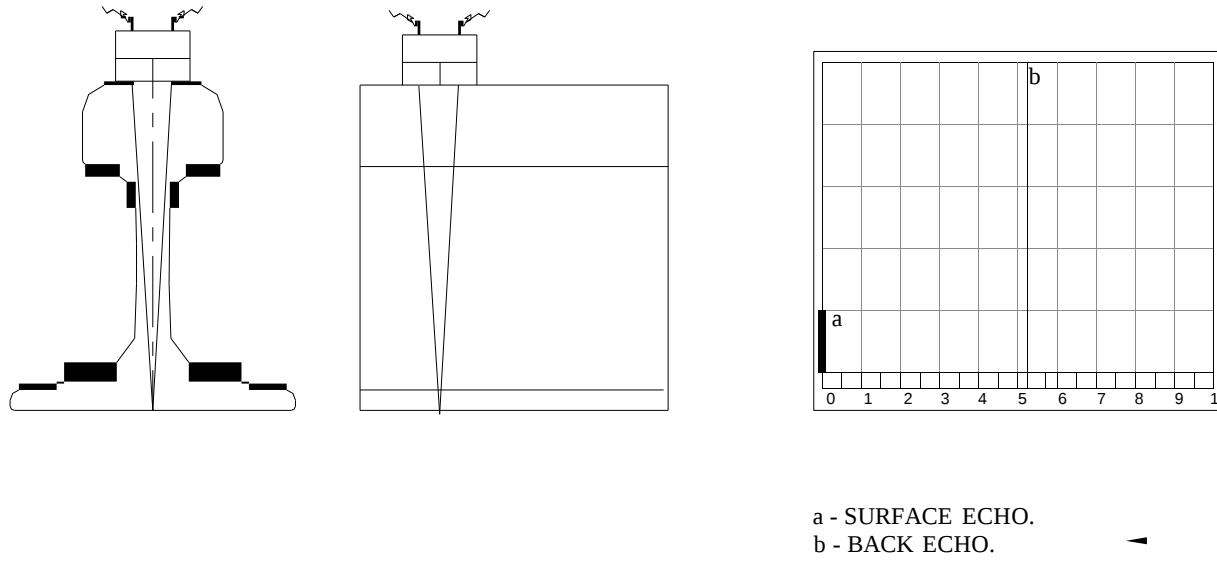
FIG.5: RAIL WITHOUT FLAW (0° PROBE)
