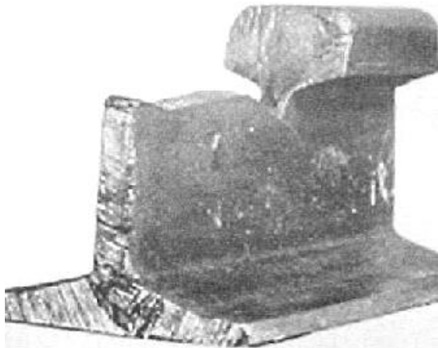
FIG. 49 : 302 -DAMAGE TO RAIL BY BAD MACHINING , DRILLING OR FLAME CUTTING
