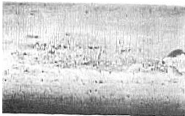
FIG. 40 : 2252 - HEAD SURFACE, WHEEL BURN REPEATED
