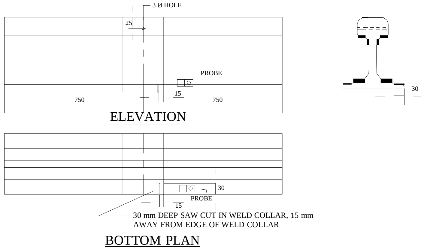
FIG. 20(b): STANDARD A.T. WELDED RAIL PIECE WITH ARTIFICIAL FLAWS FOR SENSITIVITY SETTING OF ULTRASONIC EQUIPMENT TO EXAMINE 75 MM WIDE GAP A.T. WELDS
