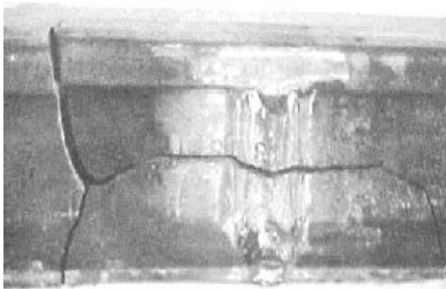
FIG. 52 : 422 - WELDING, THERMIT JOINT HORIZONTAL CRACK
