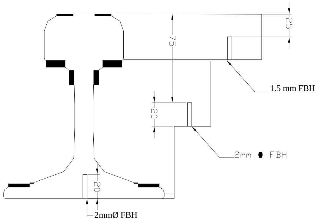
FIG. 25: STANDARD TEST RAIL PIECE FOR TESTING OF RAILS BEFORE MANUFACTURING OF POINTS & CROSSINGS
