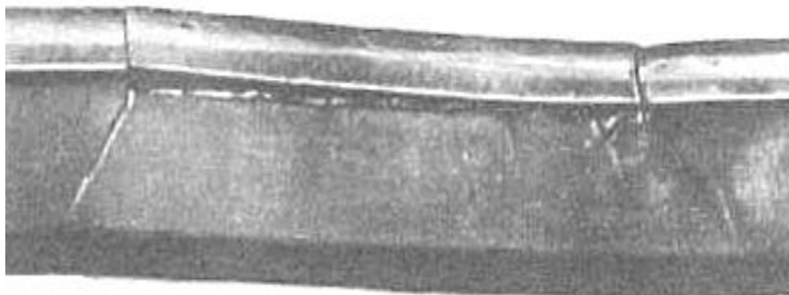
FIG. 42 : 1321 OR 2321 - WEB , HORIZONTAL CRACK, AT TOP FILLET RADIUS
