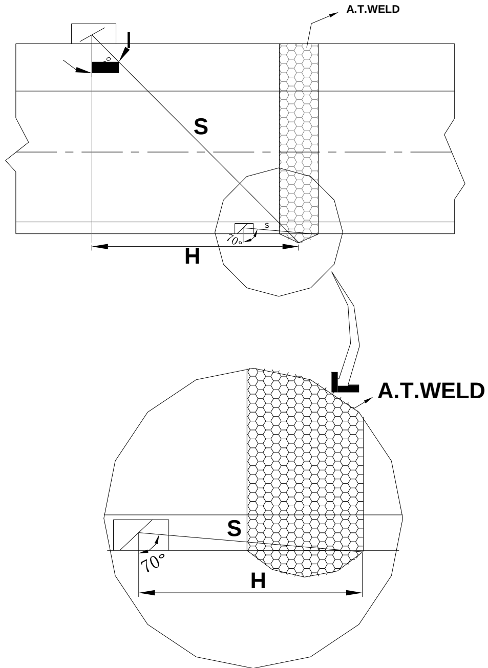
FIG. 21(b): TESTING OF BOTTOM FLANGE OF A.T. WELDS USING 70° AND 45° PROBES
