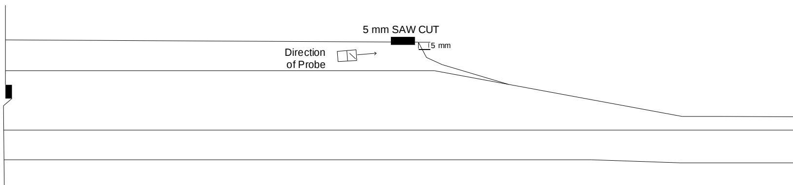
FIG.29 SENSITIVITY SETTING BLOCK & ULTRASONIC SCANNING OF TONGUE RAIL OF SEJ (RAIL IN PLAN)
