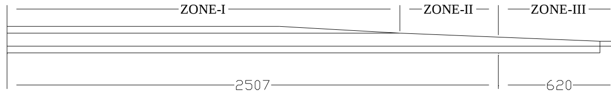
FIG. 26(a): TESTING PROCEDURE FOR POINT AND SPLICE RAILS FOR 1 IN 12 CROSSING B G 52 Kg
