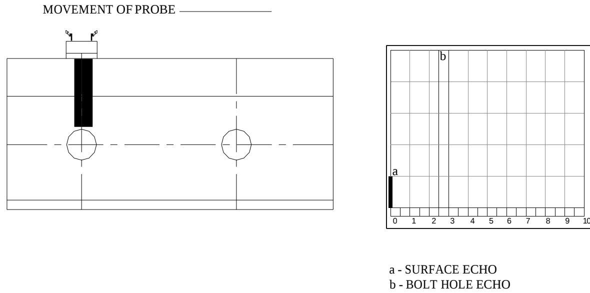
FIG. 15 : BOLT HOLE WITHOUT CRACK (0° PROBE)
